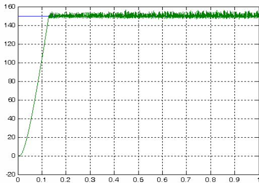
Fig. 11 Speedof the asynchronous machine with the application of the fuzzy control
