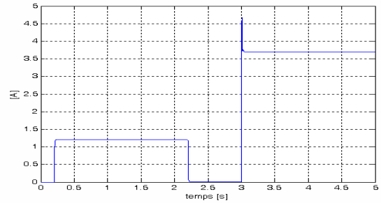
Fig. 13 Allure i_{sq} current corresponding to the rotor flux
