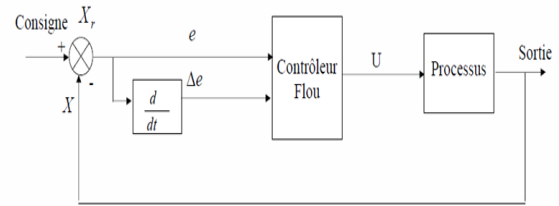
Fig.4 Architecture of the fuzzy control
