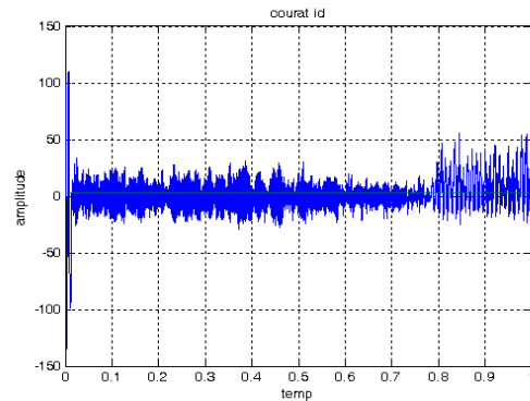
Fig. 8 i_d current of the machine controlling by PI
