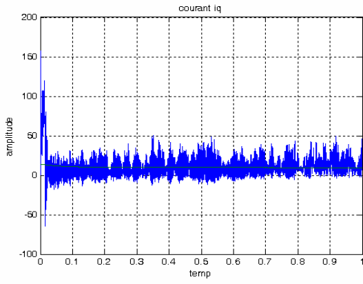
Fig. 9 i_q current of the machine controlling by PI
