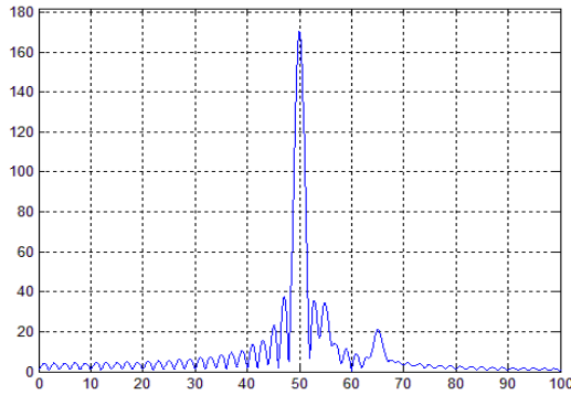
Fig. 10 Stator current spectrum
