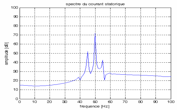
Fig. 14 Stator current spectrum of a machine with broken rotor bar
