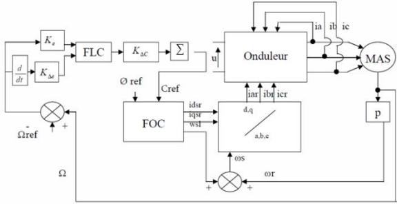
Fig.6 Adjustment structure by a fuzzy PI speed of induction machine
